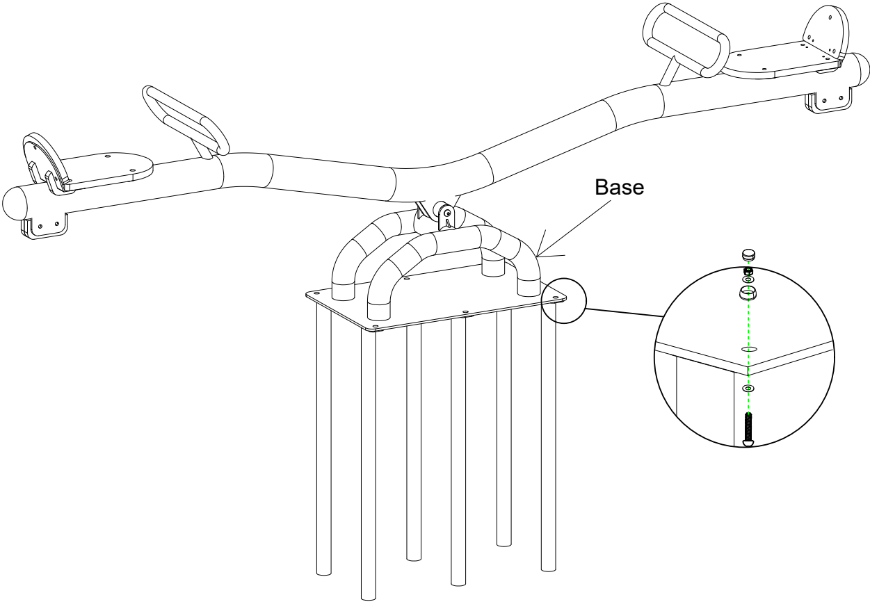
Inground Installation
